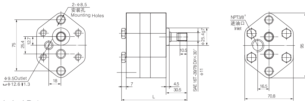
CB-G**F16
