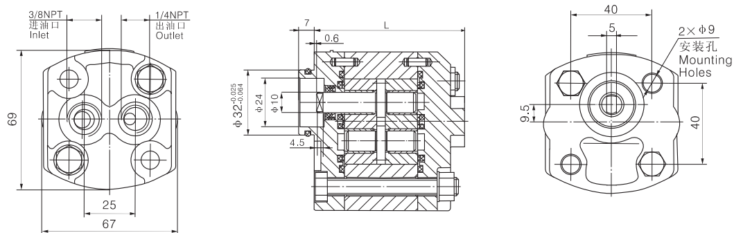
CBK1-F*DF Outline Dimension (Rear in/rear out)
