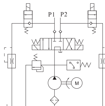
Hydraulic Circuit Diagram
